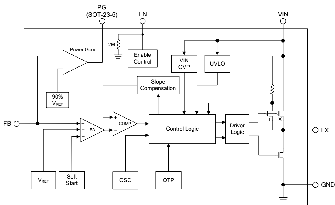
Figure 3. Block Diagram of FP6356
