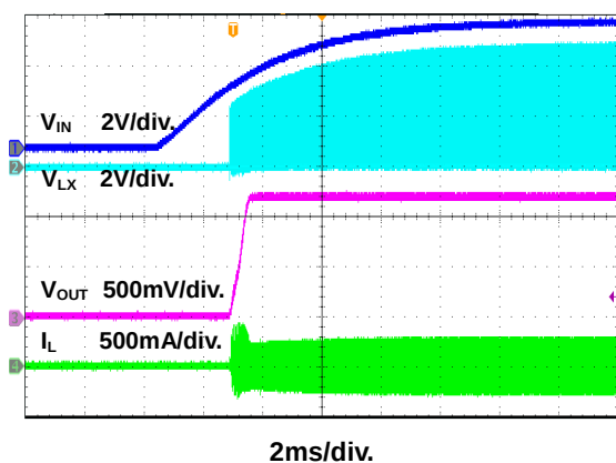
Figure 8. Power On Through VIN Waveform
