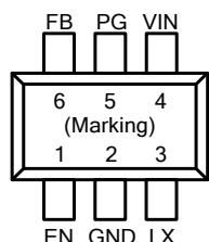
Figure 1. Pin Assignment of FP6356
