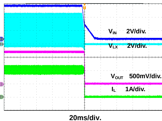
Figure 11. Power Off Through VIN Waveform
