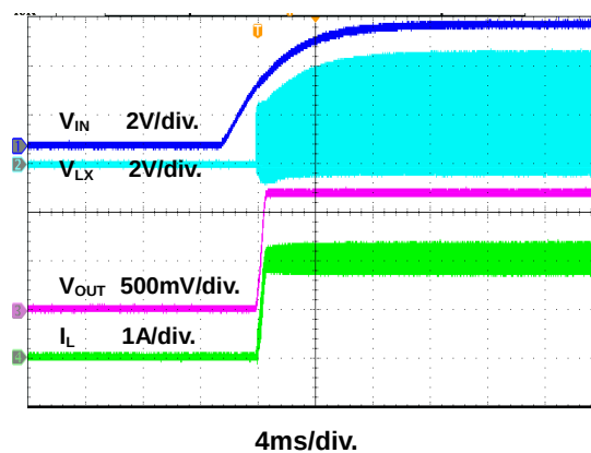
Figure 9. Power On Through VIN Waveform
