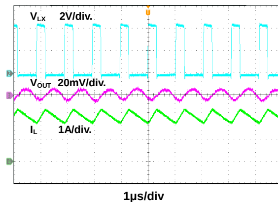
Figure 17. Steady State Waveform
