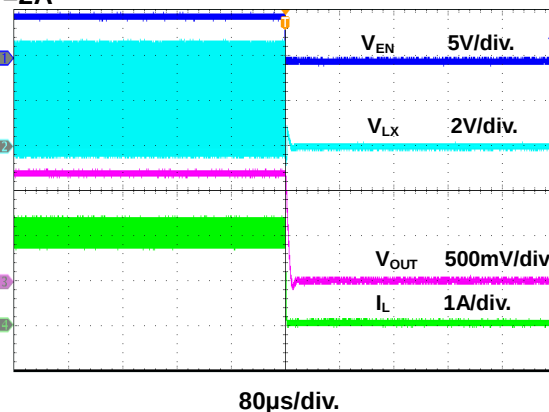
Figure 15. Power Off Through EN Waveform
