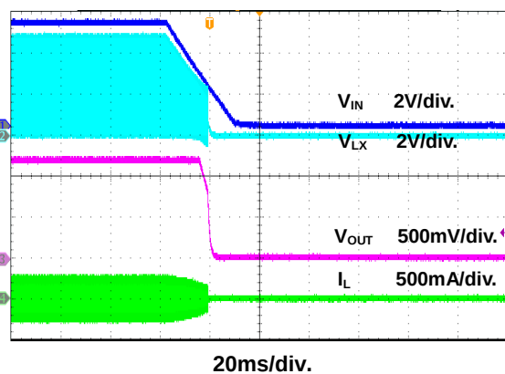
Figure 10. Power Off Through VIN Waveform
