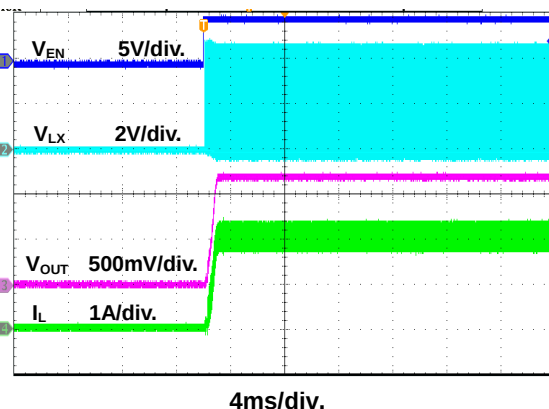
Figure 13. Power On Through EN Waveform
