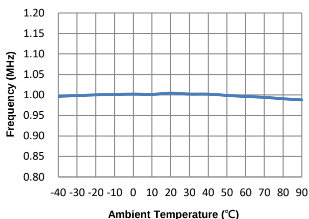
Figure 7. Frequency vs. Ambient Temperature
