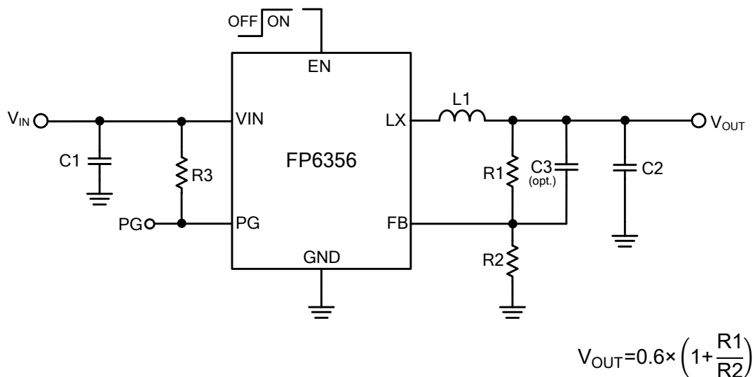
Figure 2. Schematic Diagram
