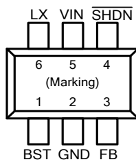
Figure 1. Pin Assignments of FR9212B
