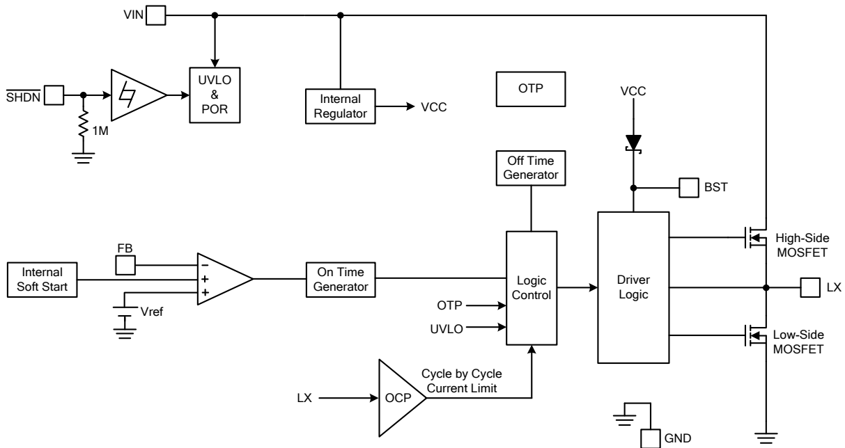
Figure 3. Block Diagram of FR9212B
