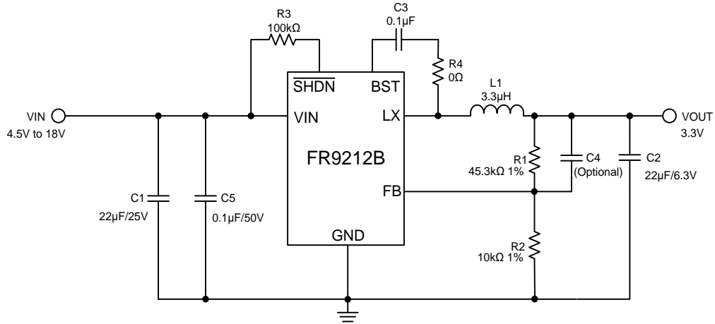
Figure 2. FR9212B Application Circuit
