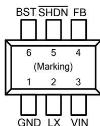
Figure 1. Pin Assignments of FR9206FH
