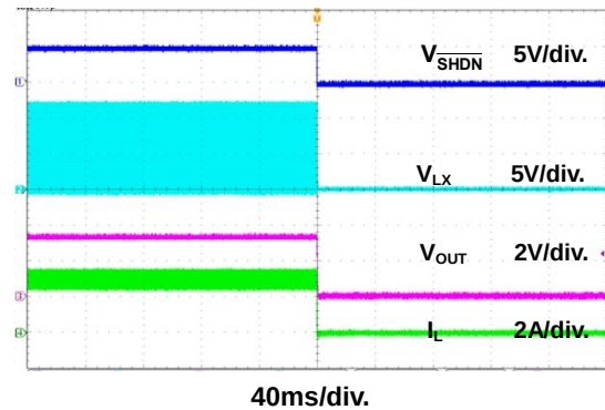
Figure 19. Power Off Through \overline{SHDN} Waveform
