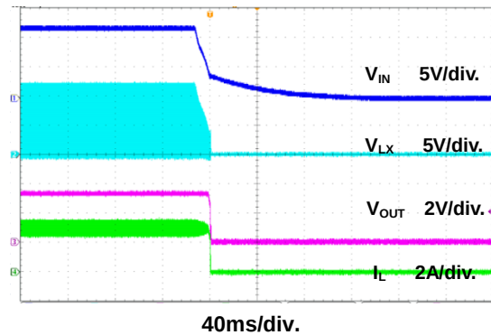
Figure 15. Power Off Through VIN Waveform
