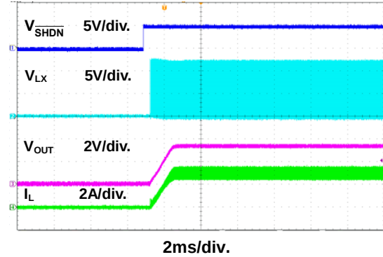
Figure 17. Power On Through \overline{SHDN} Waveform
