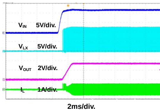
Figure 12. Power On Through VIN Waveform
