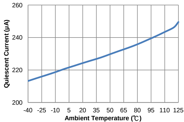
Figure 8. Quiescent Current vs. Ambient Temperature
