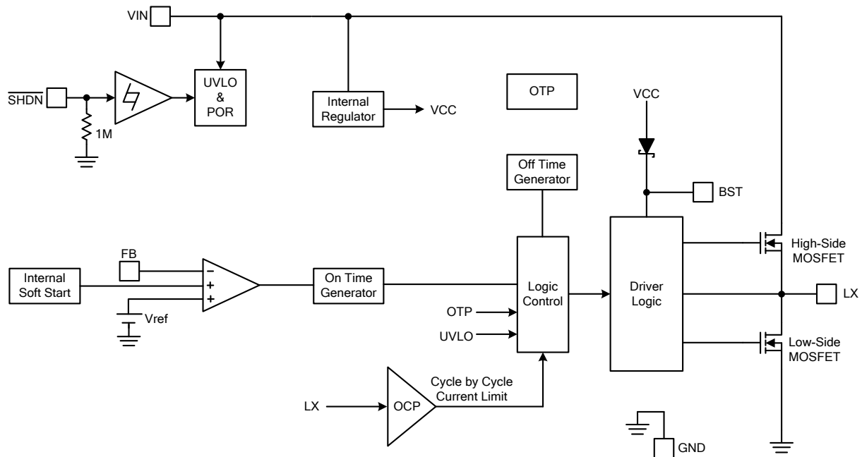
Figure 3. Block Diagram of FR9206FH
