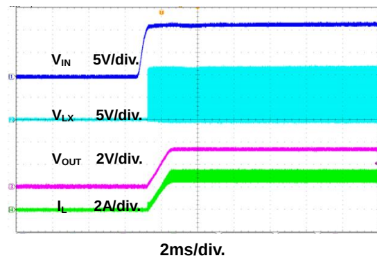
Figure 13. Power On Through VIN Waveform
