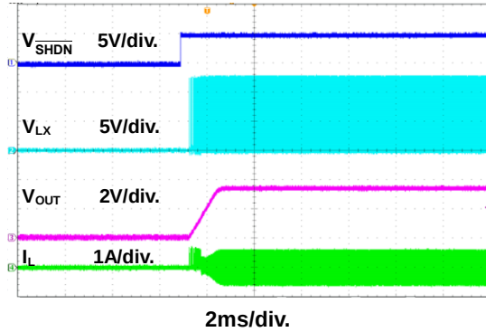
Figure 16. Power On Through \overline{SHDN} Waveform
