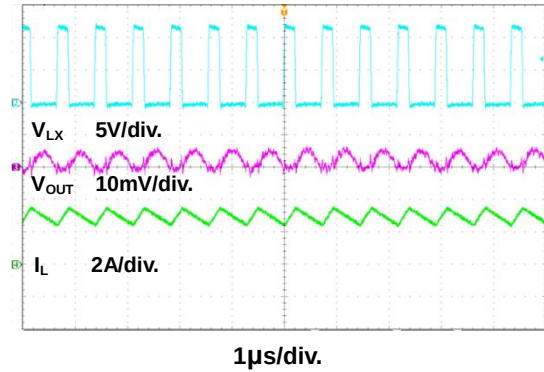
Figure 11. Steady State Waveform
