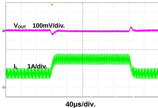
Figure 20. Load Transient Waveform
