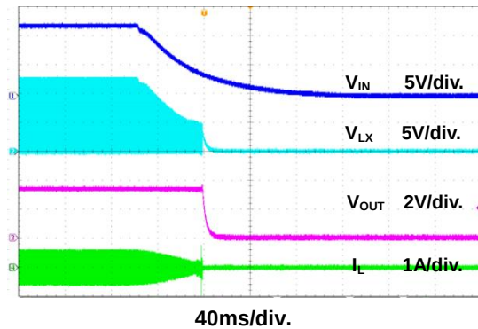
Figure 14. Power Off Through VIN Waveform
