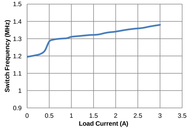
Figure 7. Switch Frequency vs. Load Current
