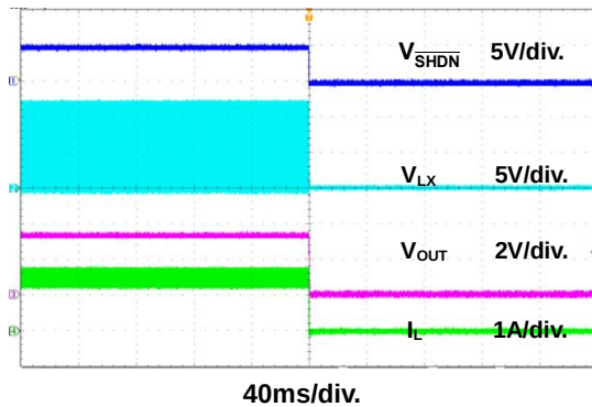
Figure 18. Power Off Through \overline{SHDN} Waveform
