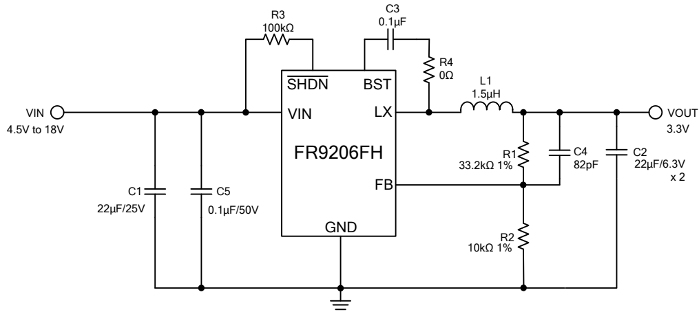
Figure 2. FR9206FH Application Circuit
