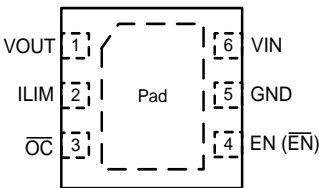
Figure1. Pin Assignment of FP6861E-A
