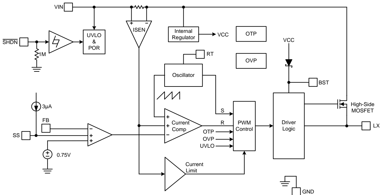
Figure 3. Block Diagram of FR9835A
