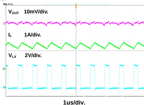
Figure 9. Steady State Waveform
