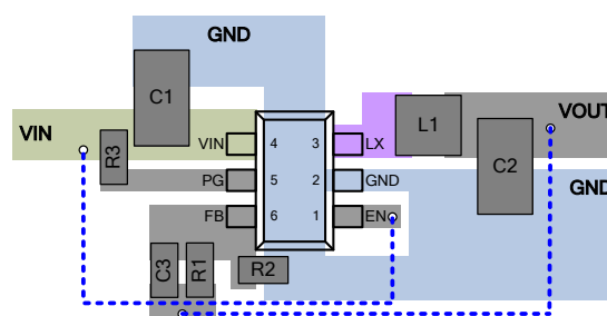
Figure 20. Recommended Layout Diagram
