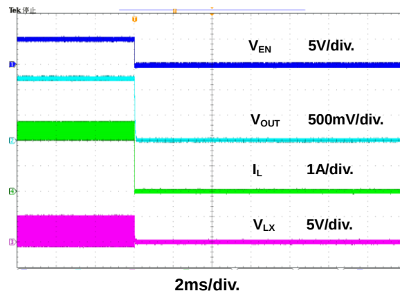
Figure 17. Power Off Through EN Waveform
