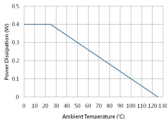
Figure 19. SOT-23-6 Package PD Derating Curve
