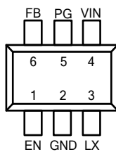
Figure 1. Pin Assignment of FP6311
