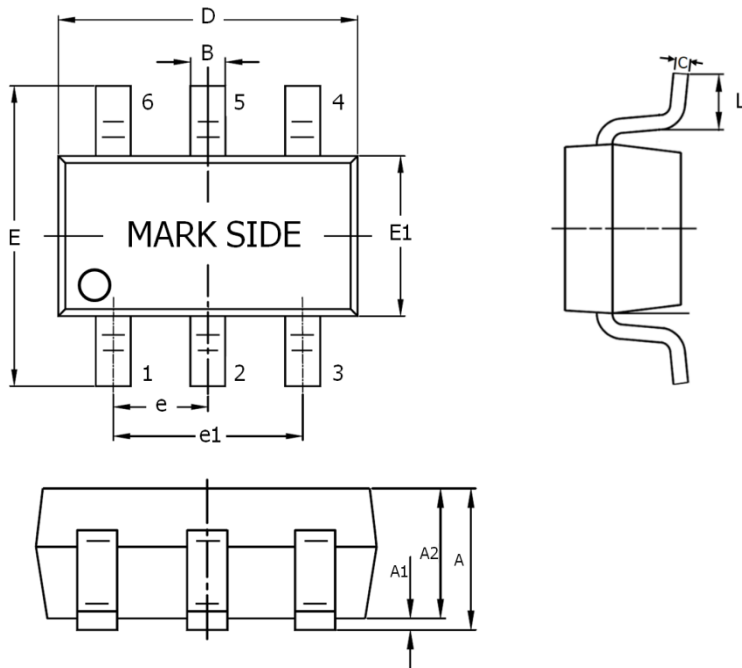
SOT-23-6L Package (Unit: mm)
