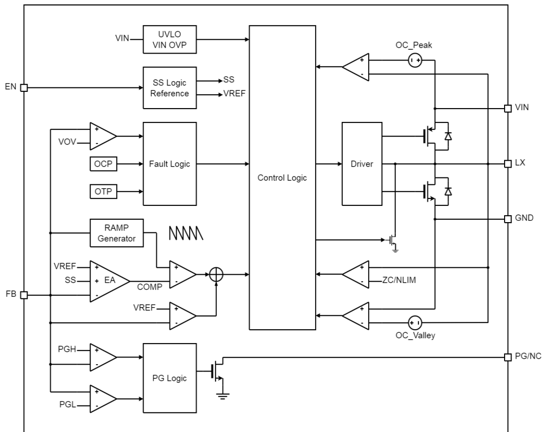
Figure 3. Block Diagram of FP6311
