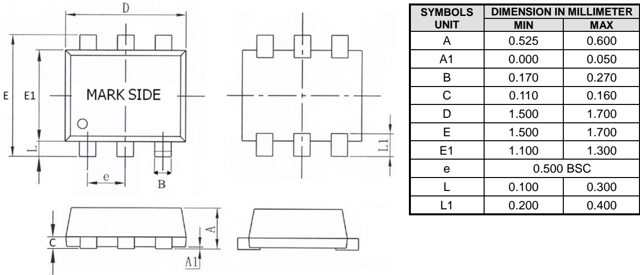
SOT-563-6L Package (Unit: mm)
