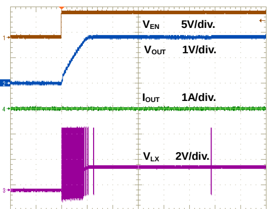
Figure 14. Power On Through EN Waveform
