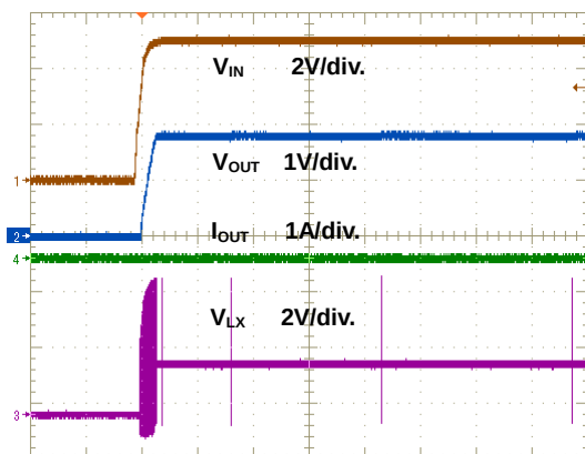
Figure 10. Power On Through VIN Waveform
