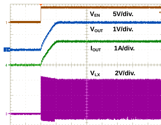
Figure 15. Power On Through EN Waveform
