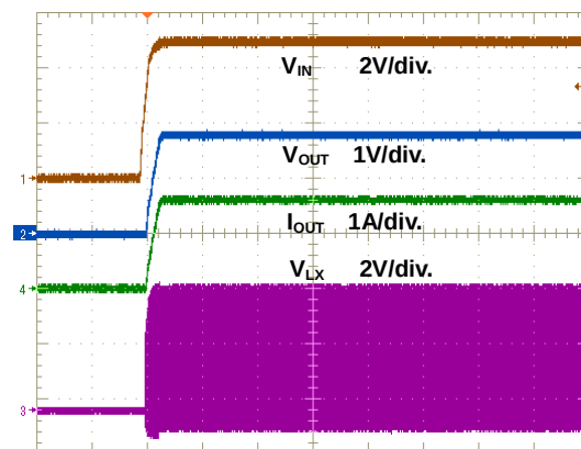
Figure 11. Power On Through VIN Waveform
