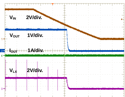
Figure 12. Power Off Through VIN Waveform
