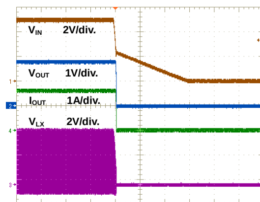
Figure 13. Power Off Through VIN Waveform
