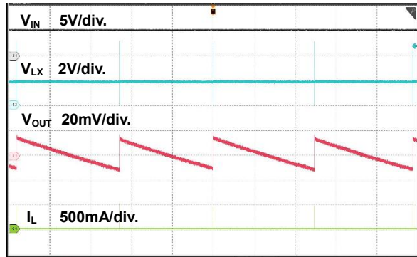
Figure 10. Steady State Waveform
