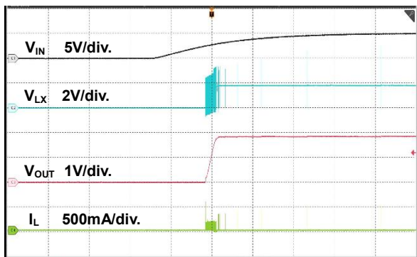
Figure 12. Power On Through V_{IN} Waveform
