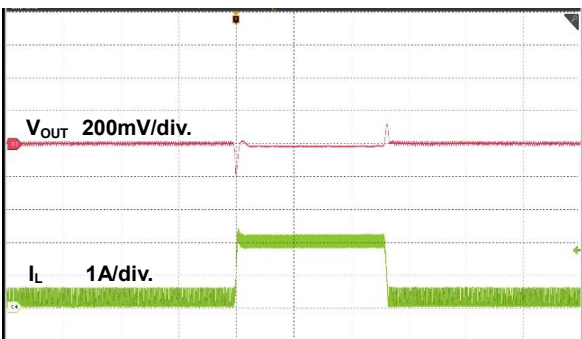
Figure 20. Load Transient Waveform
