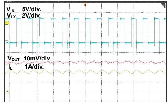
Figure 11. Steady State Waveform
