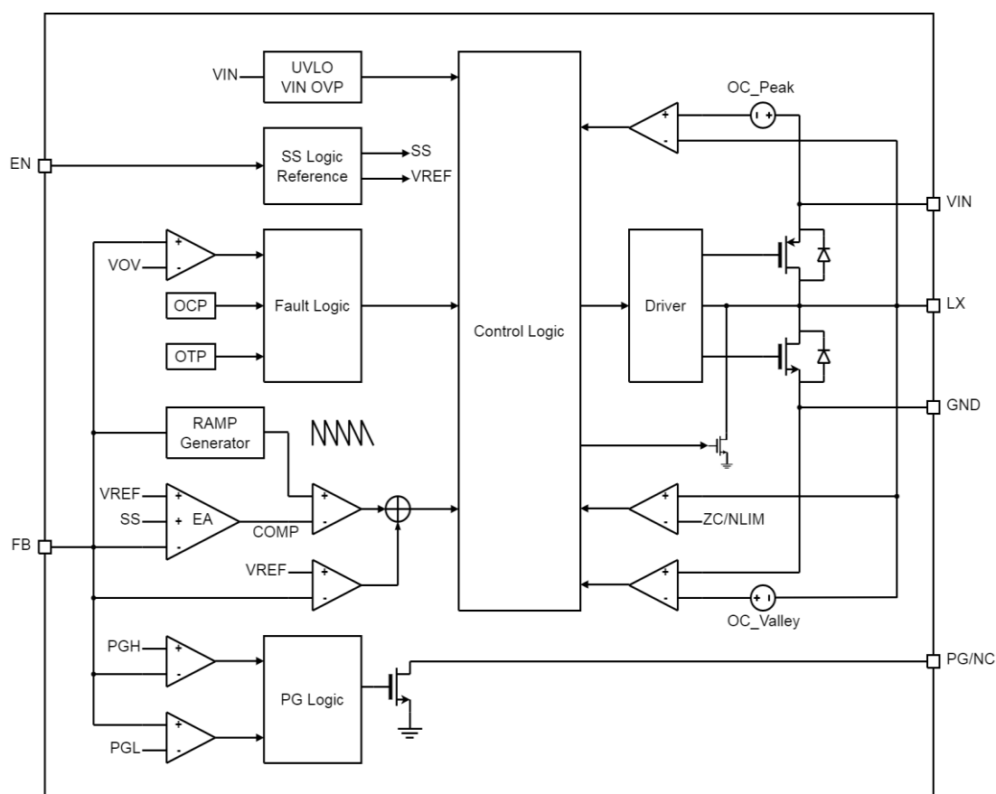
Figure 3. Block Diagram of FP6312
