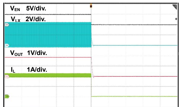
Figure 19. Power Off Through EN Waveform
