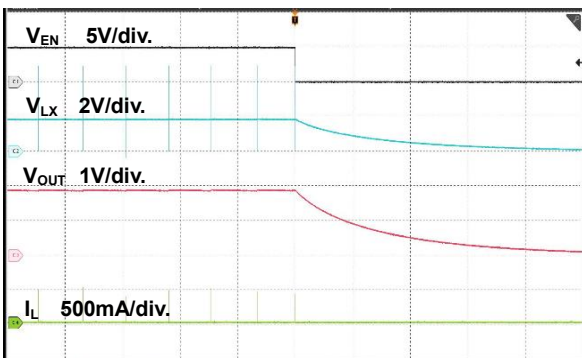
Figure 18. Power Off Through EN Waveform
