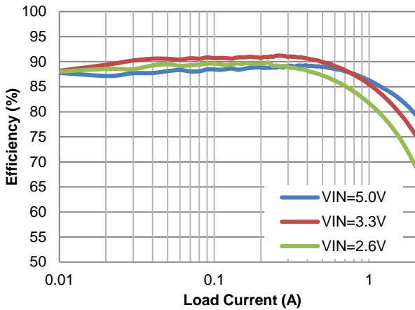
Figure 4. Efficiency vs. Load Current (SOT-563-6L)
