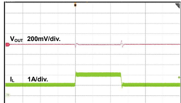
Figure 21. Load Transient Waveform
