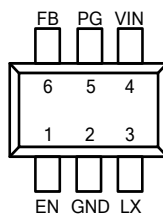
Figure 1. Pin Assignment of FP6312
