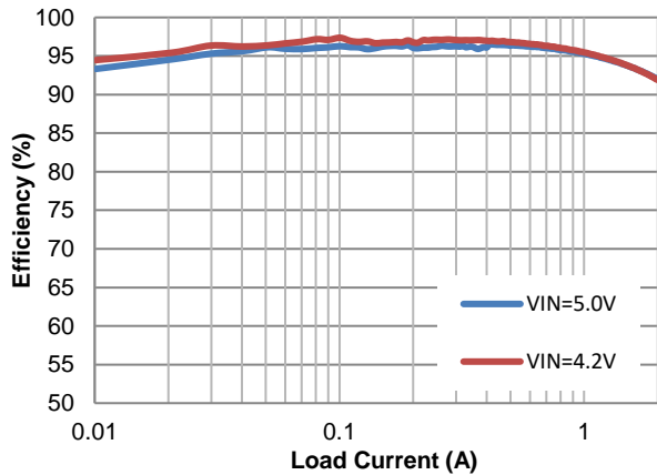
Figure 6. Efficiency vs. Load Current (SOT-563-6L)
