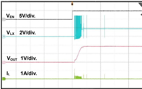
Figure 16. Power On Through EN Waveform
