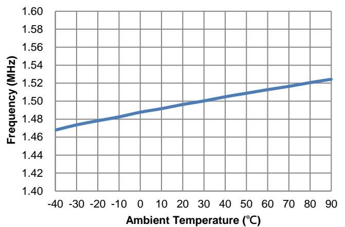
Figure 9. Frequency vs. Ambient Temperature
