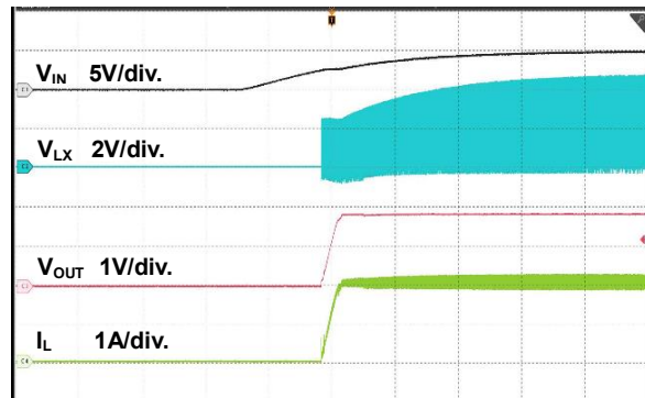
Figure 13. Power On Through V_{IN} Waveform
