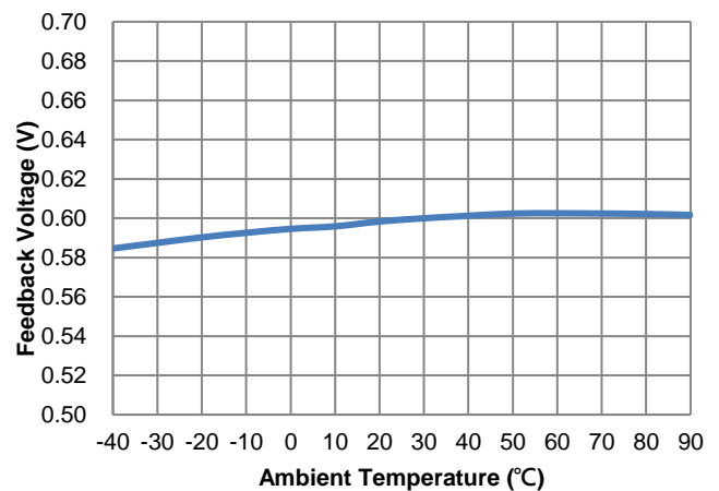
Figure 7. Feedback Voltage vs. Ambient Temperature
