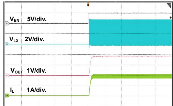
Figure 17. Power On Through EN Waveform
