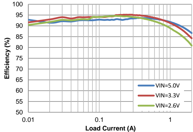
Figure 5. Efficiency vs. Load Current (SOT-563-6L)
