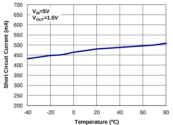
Figure 7. Short Circuit Current vs. Temperature
