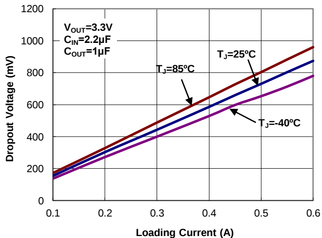
Figure 13. Dropout Voltage vs. Loading Current
