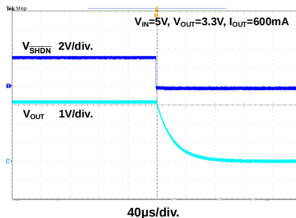
Figure 19. Shutdown Test
