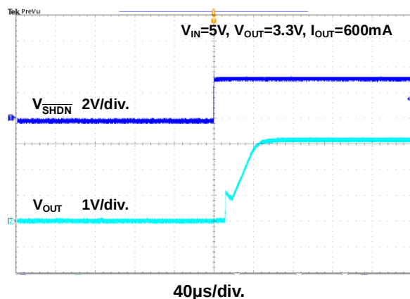
Figure 18. Enable Test
