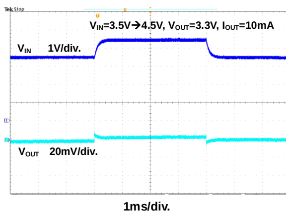
Figure 21. Line Transition Response
