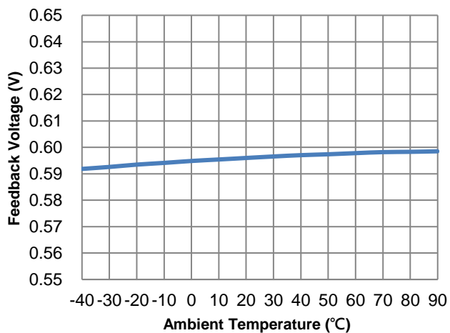
Figure 6. Feedback Voltage vs. Ambient Temperature
