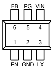
Figure 1. Pin Assignment of FP6397
