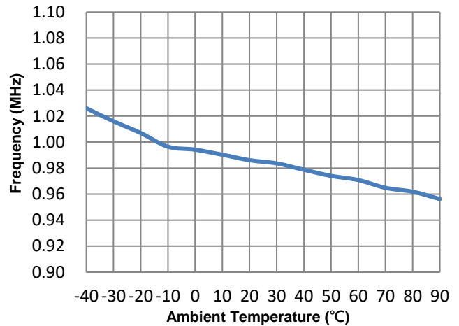
Figure 7. Frequency vs. Ambient Temperature
