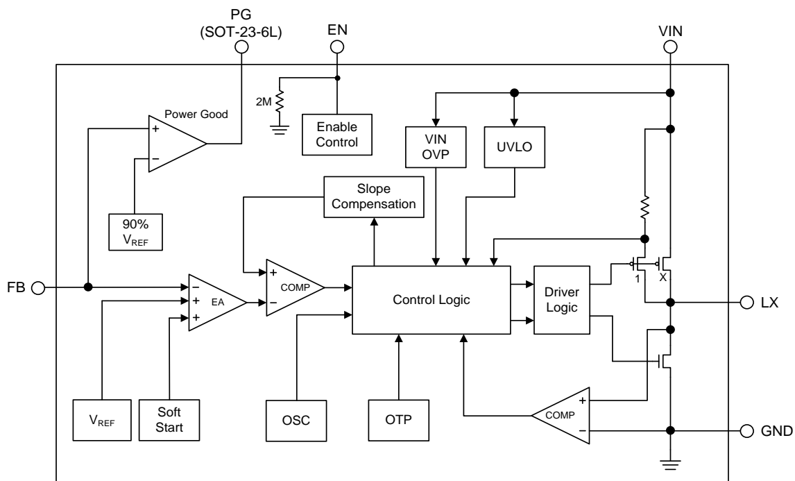
Figure 3. Block Diagram of FP6397
