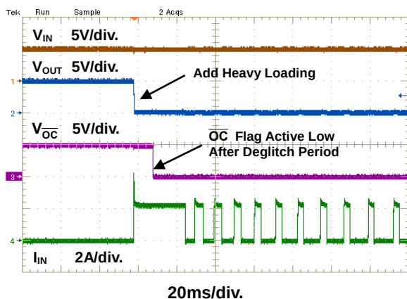
Figure 9. Short Circuit Transient Response
