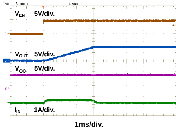
Figure 5. EN Start Up with No Load
