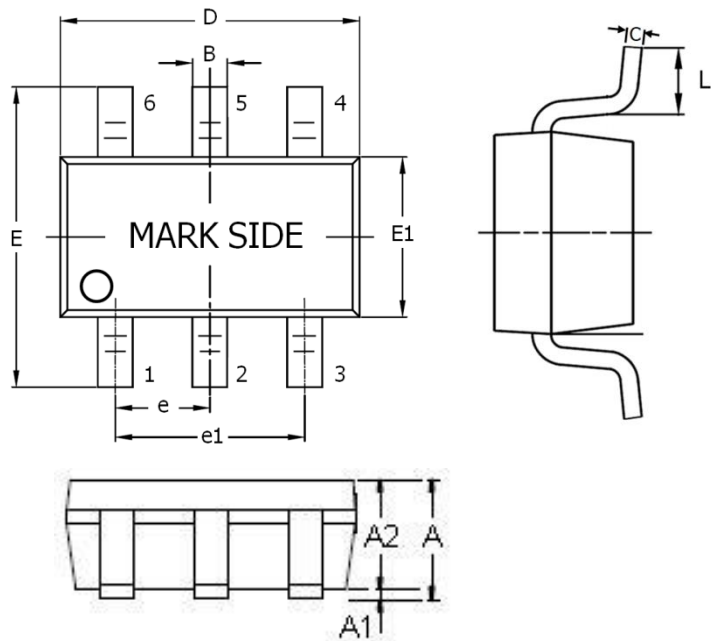
SOT-23-6L Package (Unit: mm)
