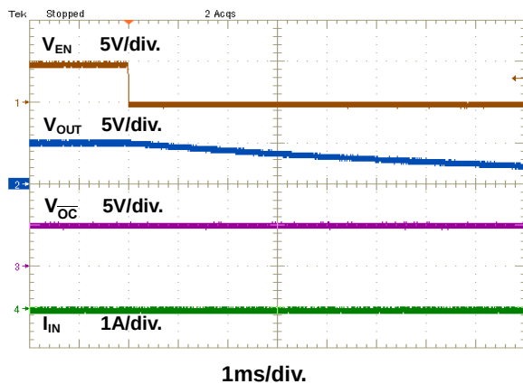
Figure 7. EN Power Off with No Load
