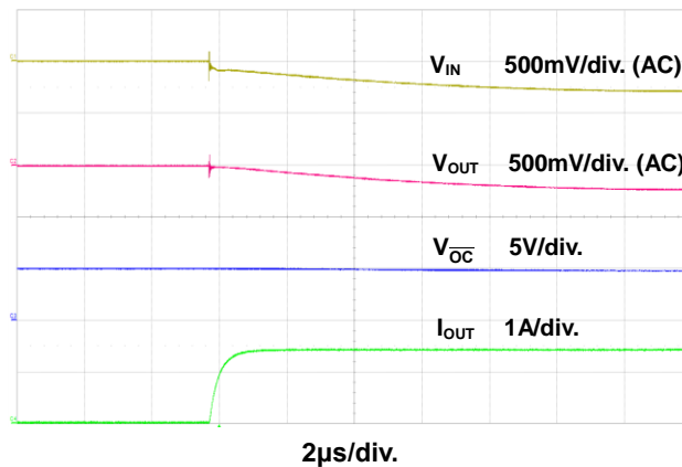
Figure 11. Output Load Insert Hot Plug-In with 3.1\Omega (1.6A)
