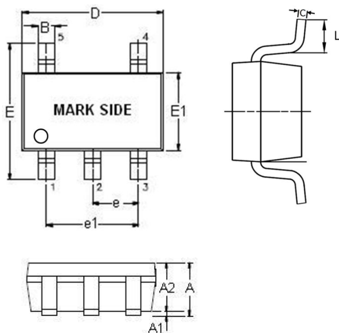
SOT-23-5 Package (Unit: mm)
