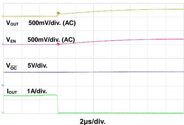
Figure 12. Output Load Insert Hot Plug-Off with 3.1\Omega (1.6A)
