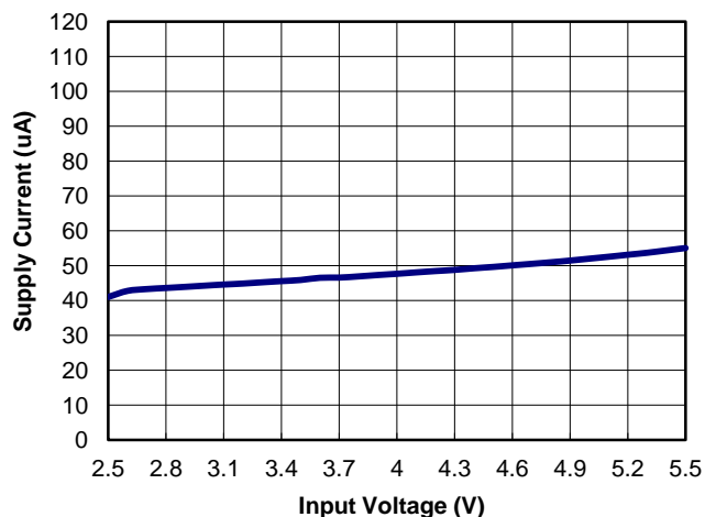
Figure 14. Supply Current vs. Input Voltage
