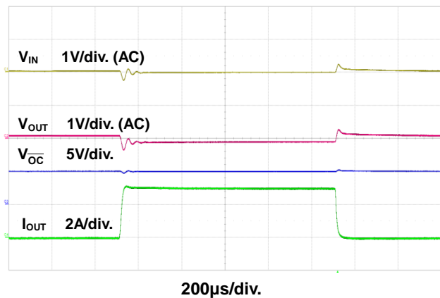
Figure 10. Load Transient
