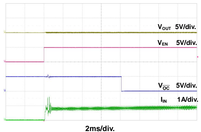
Figure 9. Short Circuit Response at Start Up
