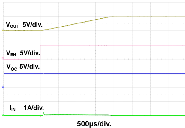
Figure 4. EN Start-Up
