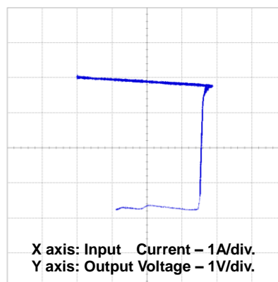
Figure 11. Output Load Insert Hot Plug-In with 3.1\Omega (1.6A)
