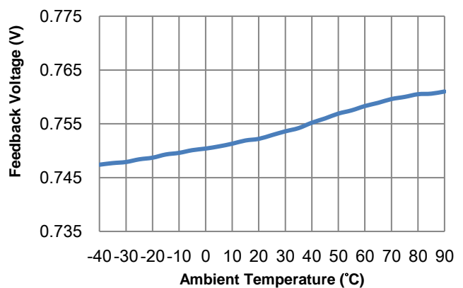
Figure 9. Feedback Voltage vs. Ambient Temperature
