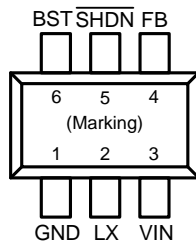
Figure 1. Pin Assignments of FR9212A
