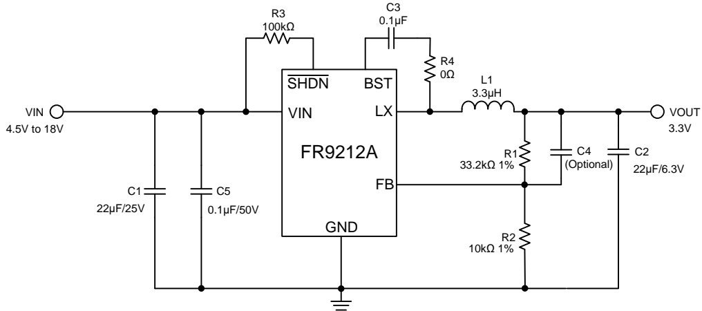
Figure 2. FR9212A Application Circuit
