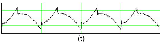
V_{\text{RIPPLE}}(t)
