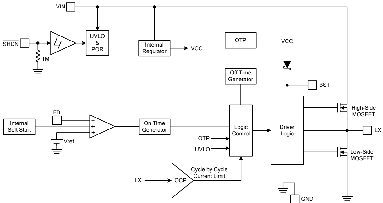
Figure 3. Block Diagram of FR9212A
