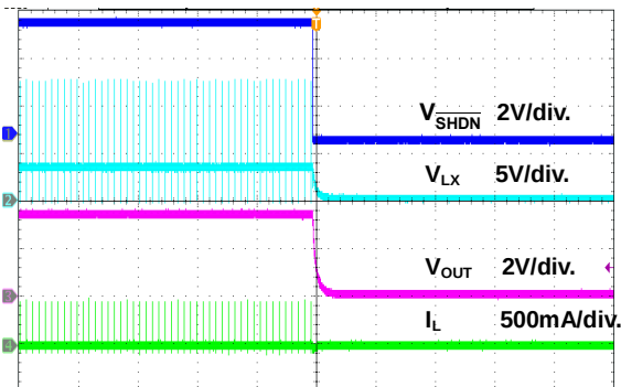
Figure 18. Shutdown Through \overline{SHDN} Waveform
