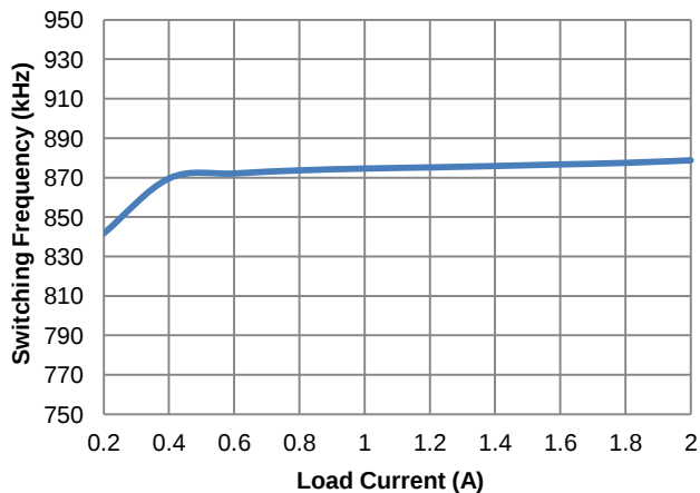
Figure 8. Switching Frequency vs. Load Current
