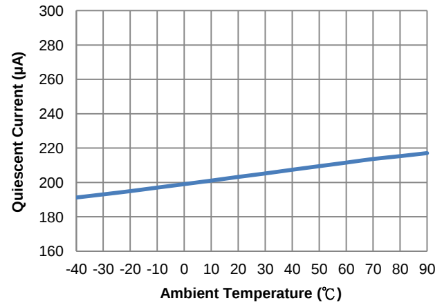
Figure 7. Quiescent Current vs. Ambient Temperature
