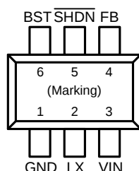
Figure 1. Pin Assignments of FR9205
