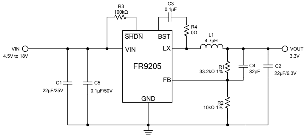
Figure 2. FR9205 Application Circuit
