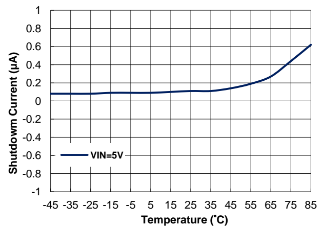
Figure 19. Shutdown Current vs. Temperature
