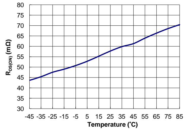
Figure 21. R_{DS(ON)} vs. Temperature
