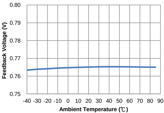
Figure 13. Feedback Voltage vs. Ambient Temperature
