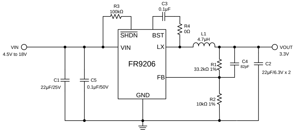
Figure 2. FR9206S9 Application Circuit
