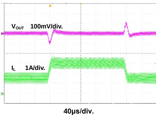
Figure 25. Load Transient Waveform
