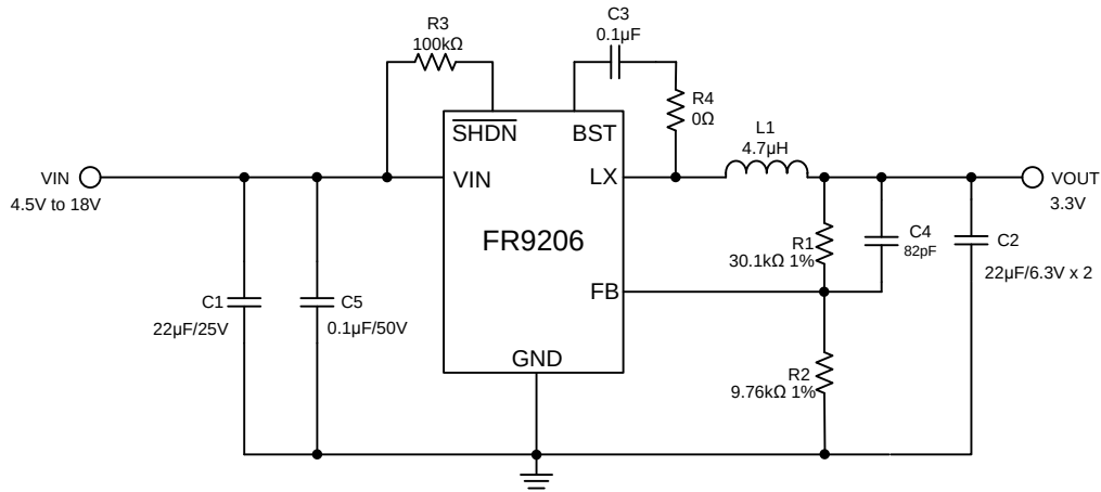
Figure 3. FR9206SD Application Circuit
