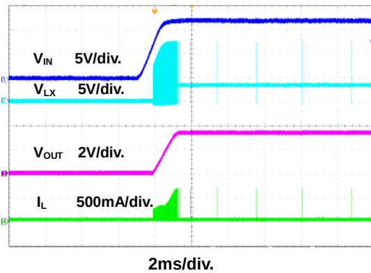
Figure 17. Power On Through VIN Waveform
