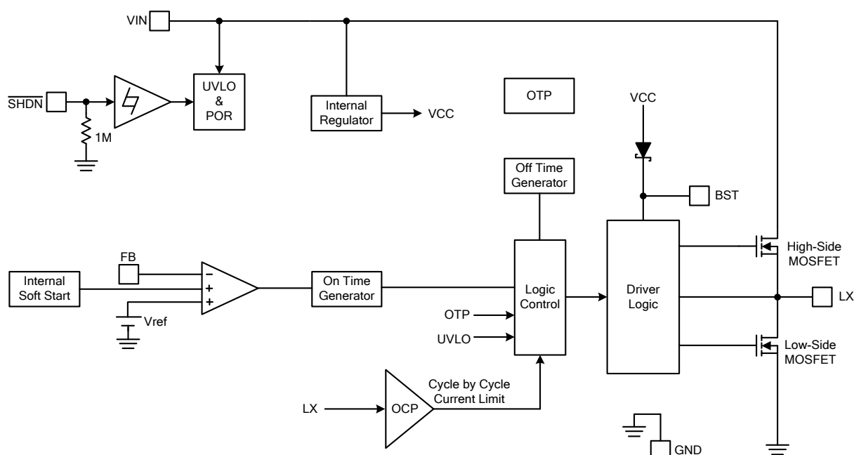
Figure 4. Block Diagram of FR9206
