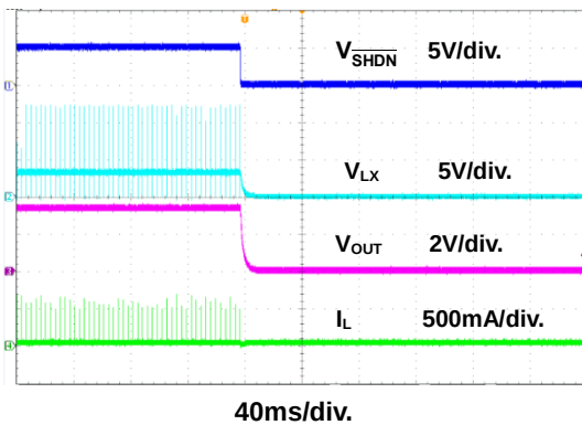
Figure 23. Power Off Through \overline{SHDN} Waveform
