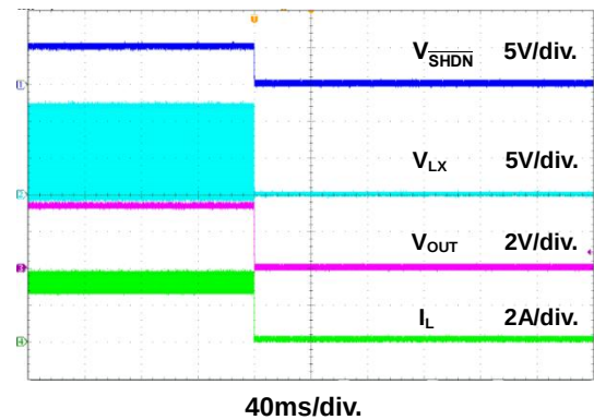
Figure 24. Power Off Through \overline{SHDN} Waveform
