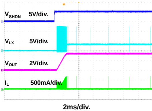
Figure 21. Power On Through \overline{SHDN} Waveform
