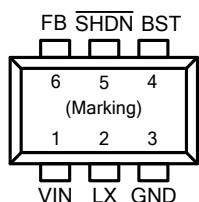
Figure 1. Pin Assignments of FR9206
