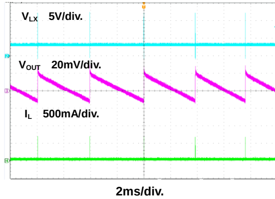
Figure 15. Steady State Waveform
