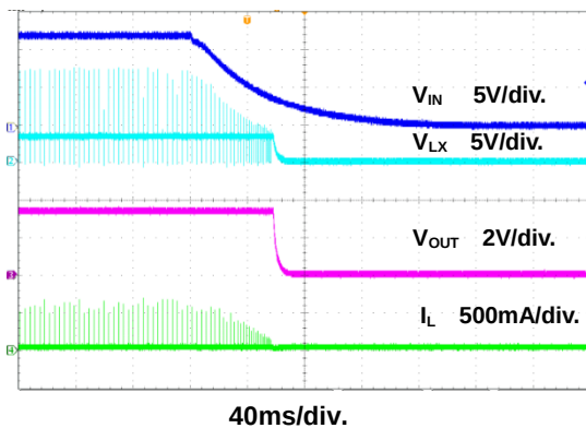
Figure 19. Power Off Through VIN Waveform
