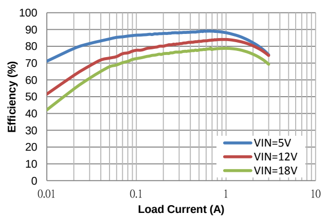
Figure 8. Efficiency vs. Load Current
