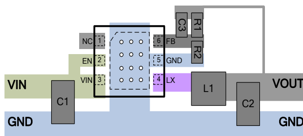
Figure 18. Recommended Layout Diagram for TDFN-6L Package
