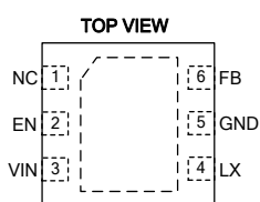
Figure 1. Pin Assignment of FP6335
