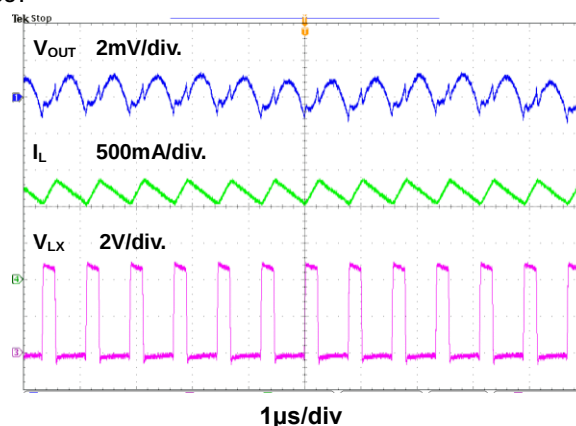
Figure 7. Steady State Waveform
