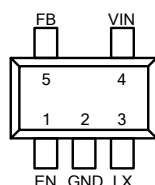
Figure 1. Pin Assignment of FP6396
