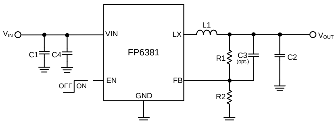
Figure 2. Schematic Diagram
