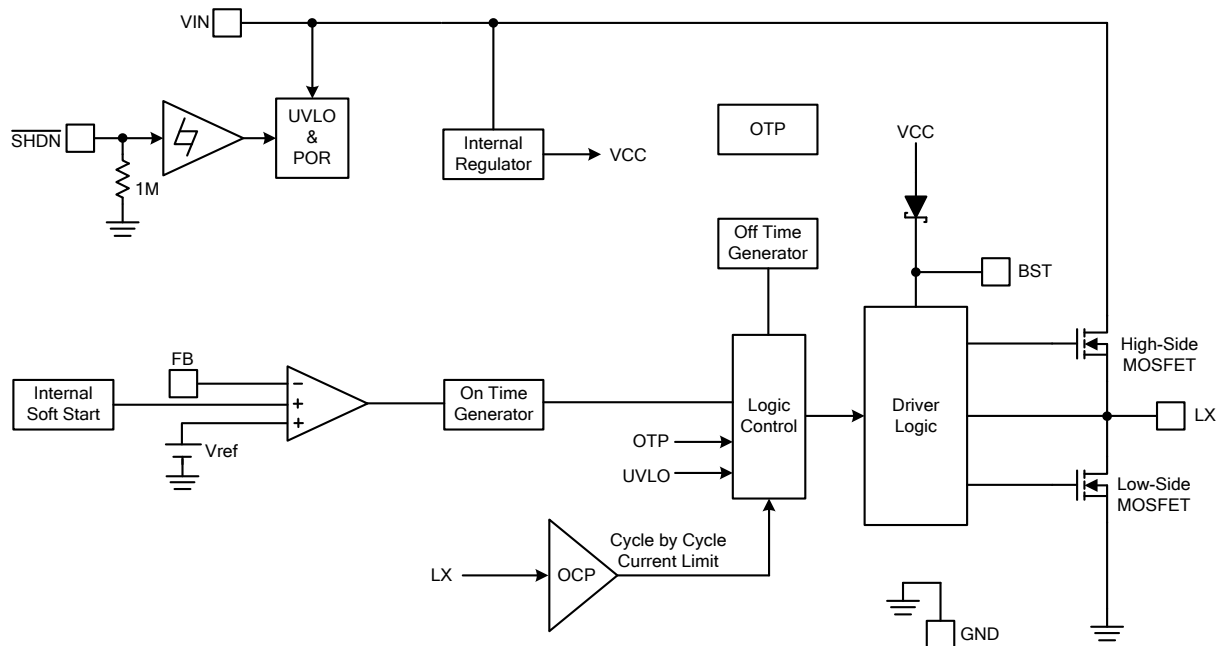
Figure 4. Block Diagram of FR9206F
