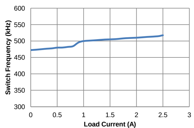
Figure 7. Switch Frequency vs. Load Current
