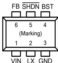
Figure 1. Pin Assignments of FR9204F
