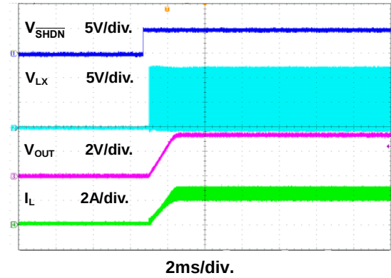
Figure 17. Power On Through \overline{SHDN} Waveform
