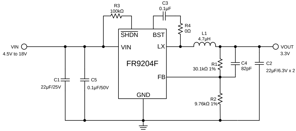
Figure 2. FR9204F Application Circuit
