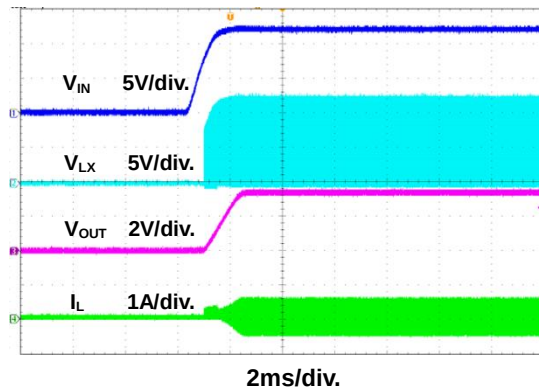
Figure 12. Power On Through VIN Waveform
