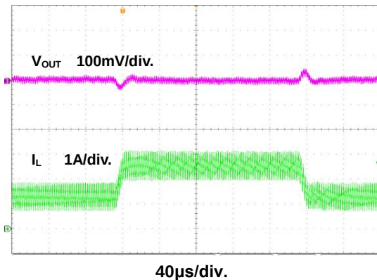
Figure 20. Load Transient Waveform
