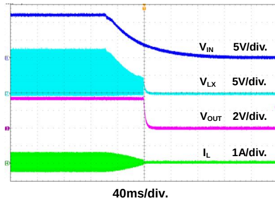
Figure 14. Power Off Through VIN Waveform
