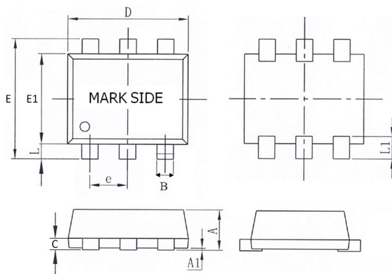
SOT-563-6L Package (Unit: mm)
