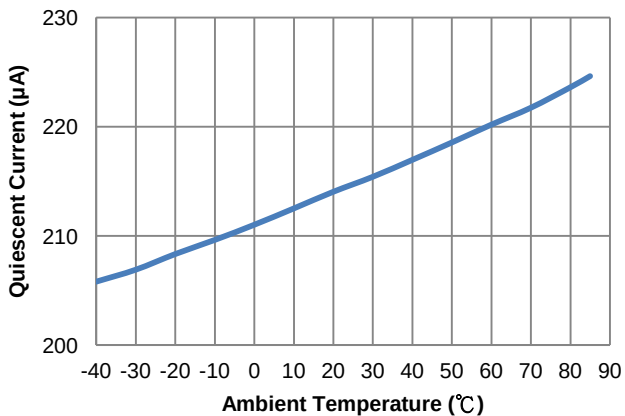
Figure 8. Quiescent Current vs. Ambient Temperature
