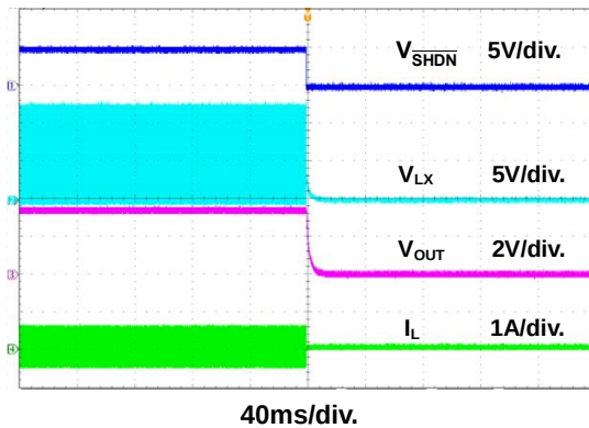
Figure 18. Power Off Through \overline{SHDN} Waveform
