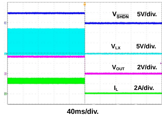
Figure 19. Power Off Through \overline{SHDN} Waveform
