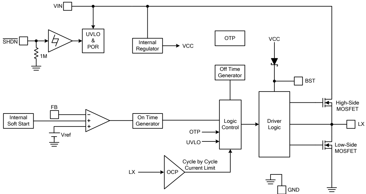
Figure 3. Block Diagram of FR9204F
