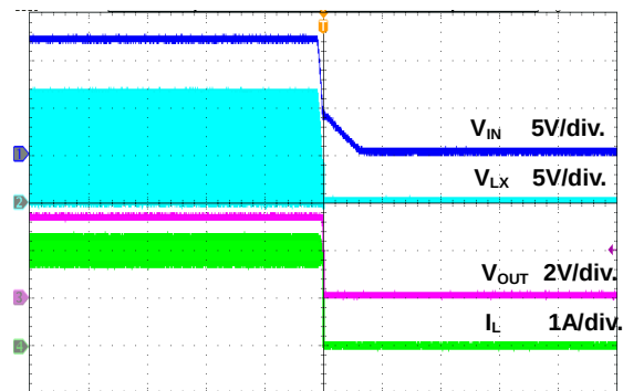
Figure 15. Shutdown Through Power Supply Waveform
