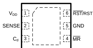
D7 Package (TDFN-6)(2mmx2mm)
