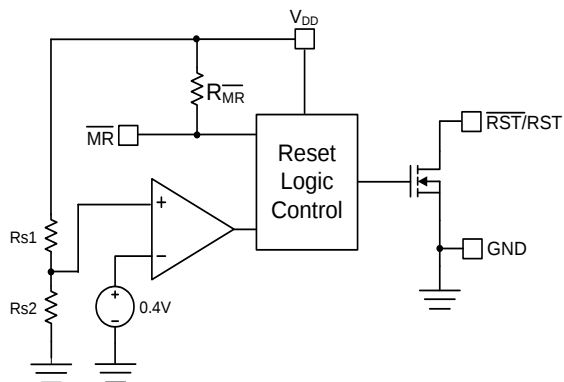
Figure 5. Adjustable Output of FP6805S9/FP6805D7
