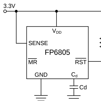
(a) Capacitor adjustable delay time
