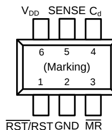
D7 Package (TDFN-6)(2mmx2mm)
