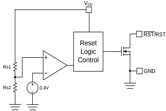
Figure 6. Fixed Output of FP6805S9
