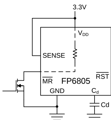
Figure 13. Applying an External NMOSFET to Minimize I_{\text{DD}} When \overline{\text{MR}} Signal does not reach V_{\text{DD}}
