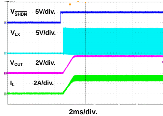
Figure 22. Power On Through \overline{SHDN} Waveform
