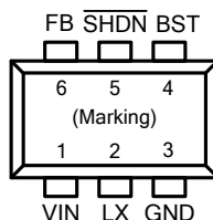
Figure 1. Pin Assignments of FR9206F
